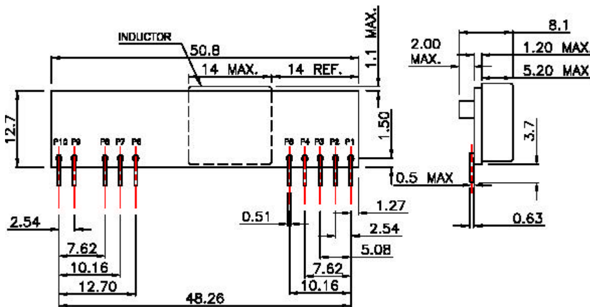
Mechanical Dimensions - Vertical type
