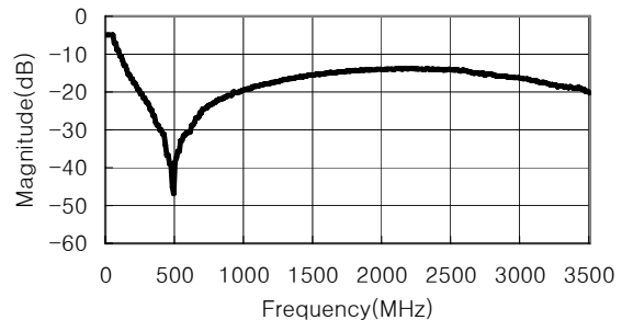
Output Return Loss vs. Frequency
