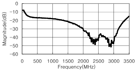
Input Return Loss vs. Frequency
