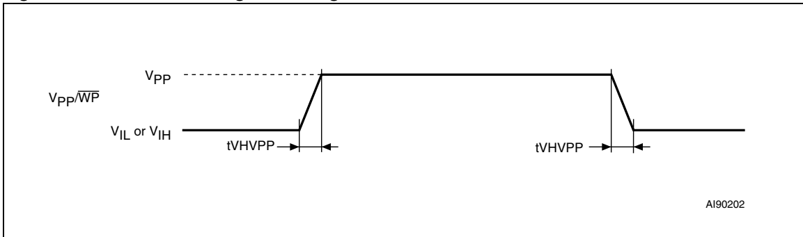
Figure 13. Accelerated Program Timing Waveforms
