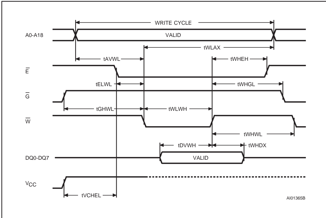
Figure 7. Write AC Waveforms, \overline{W} Controlled
