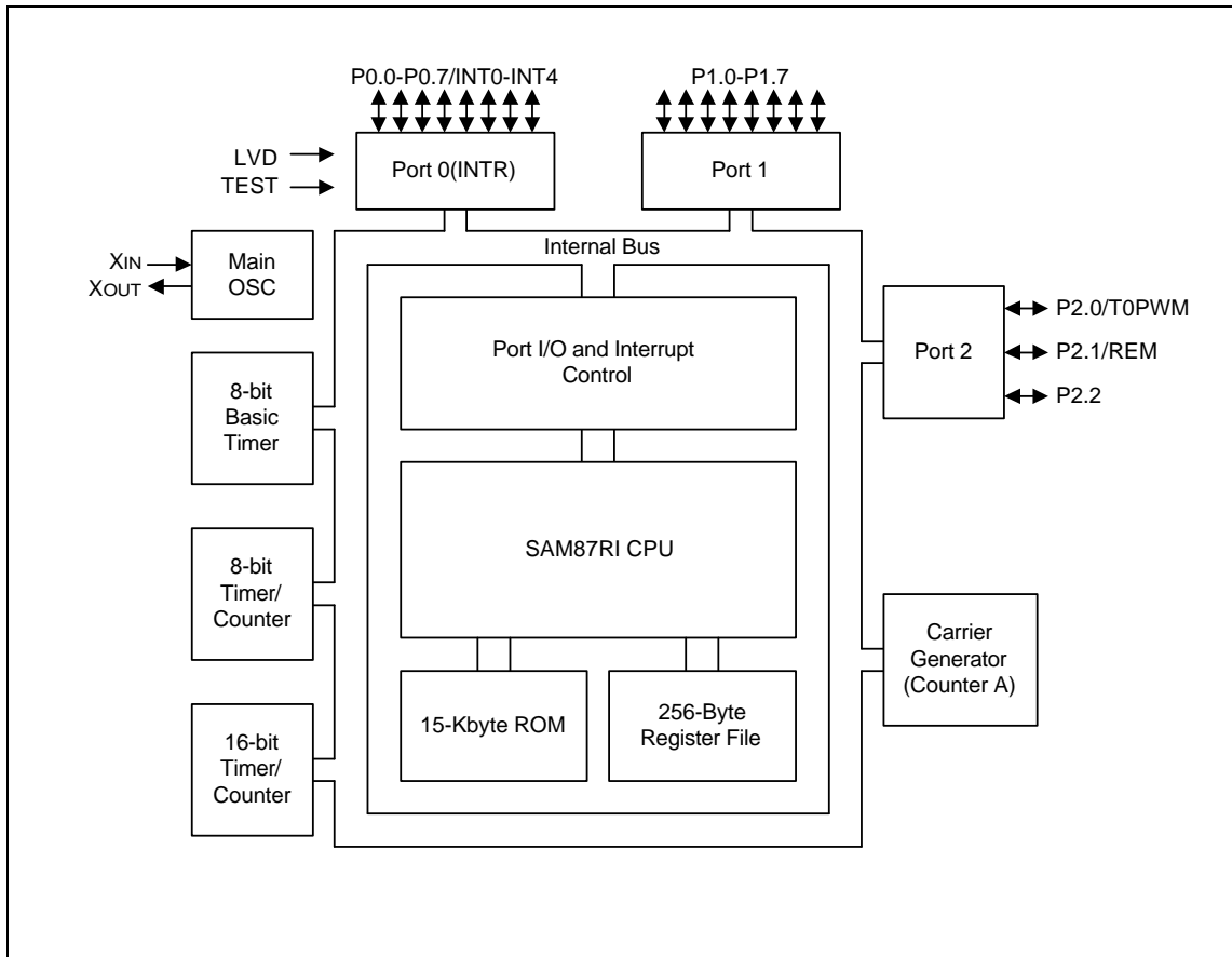
Figure 1-1. Block Diagram
