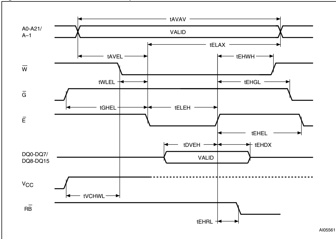
Figure 13. Write AC waveforms, Chip Enable controlled
