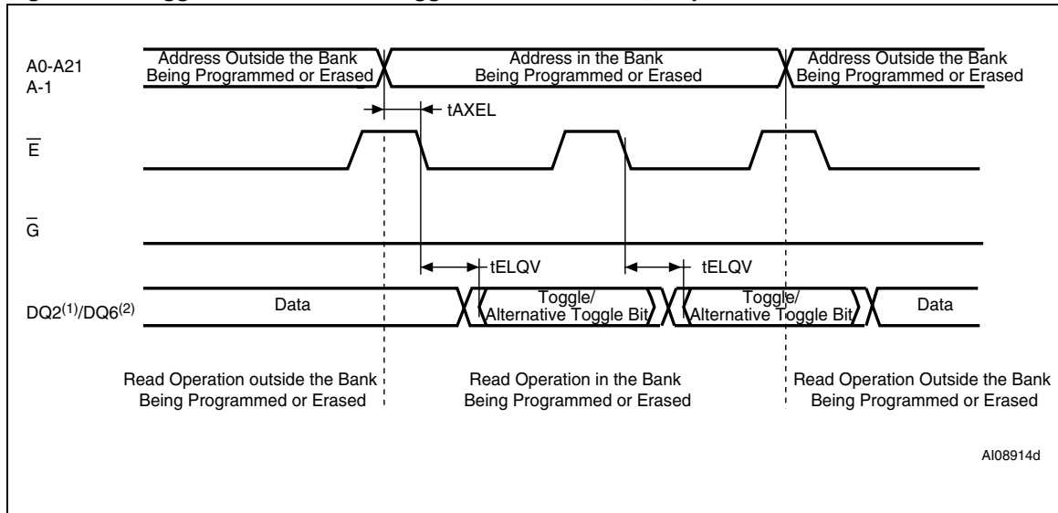
Figure 14. Toggle and Alternative Toggle Bits mechanism, Chip Enable controlled
