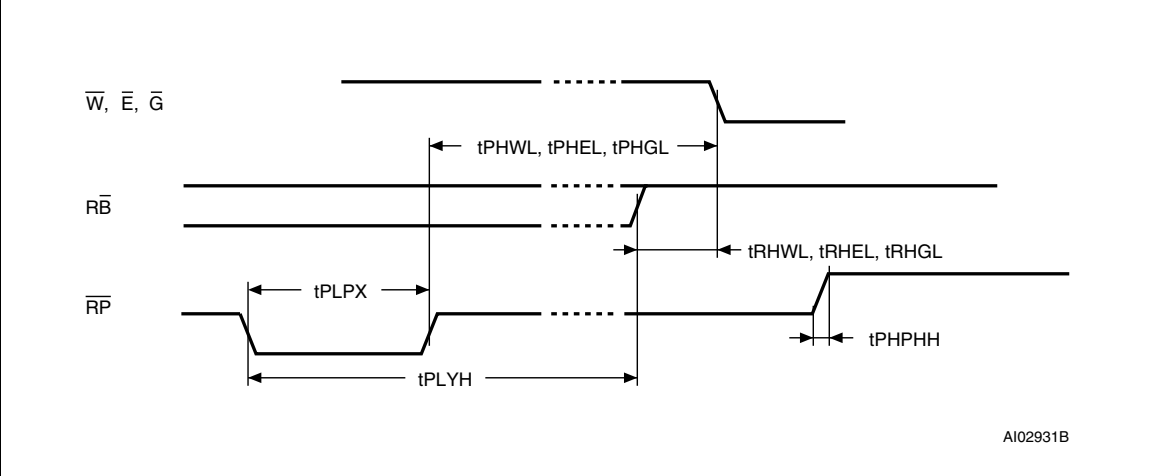
Figure 16. Reset/Block Temporary Unprotect AC waveforms
