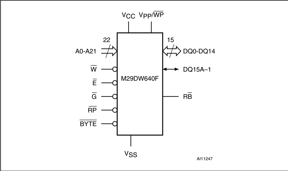
Figure 1. Logic diagram
