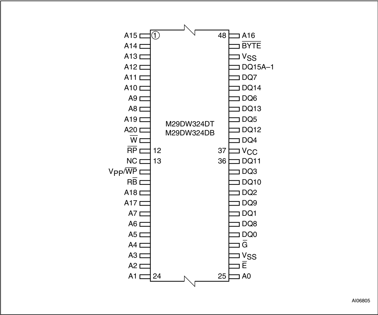
Figure 3. TSOP Connections
