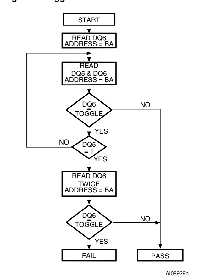
Figure 8. Toggle Flowchart
