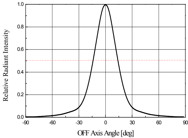
Off Axis Angle vs. Relative Intensity
