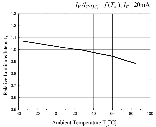
Ambient Temperature vs. Relative Intensity
