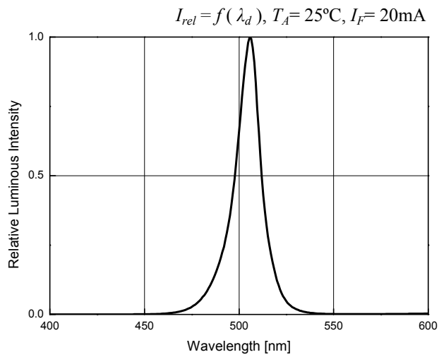
Wavelength vs. Relative Intensity
