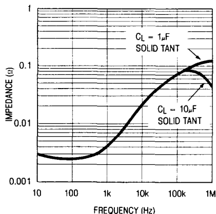
Output Impedance
