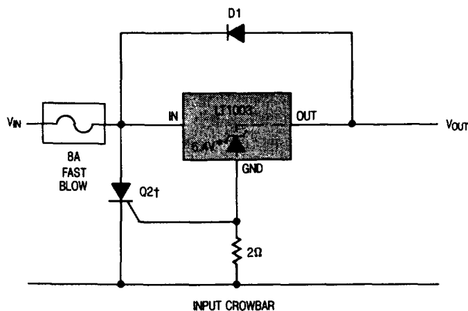
INPUT CROWBAR
