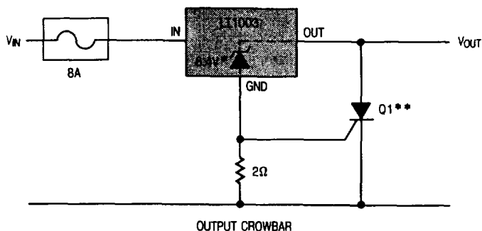
OUTPUT CROWBAR
