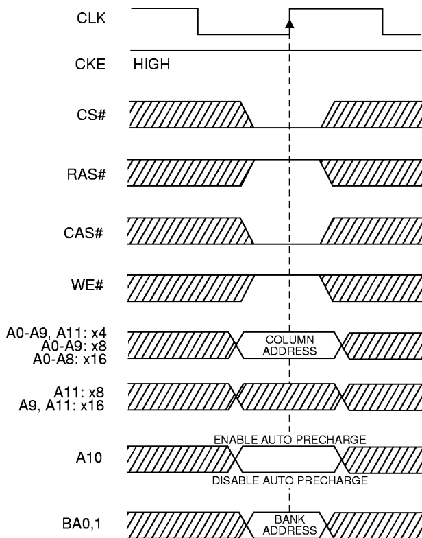
Figure 5 READ COMMAND
