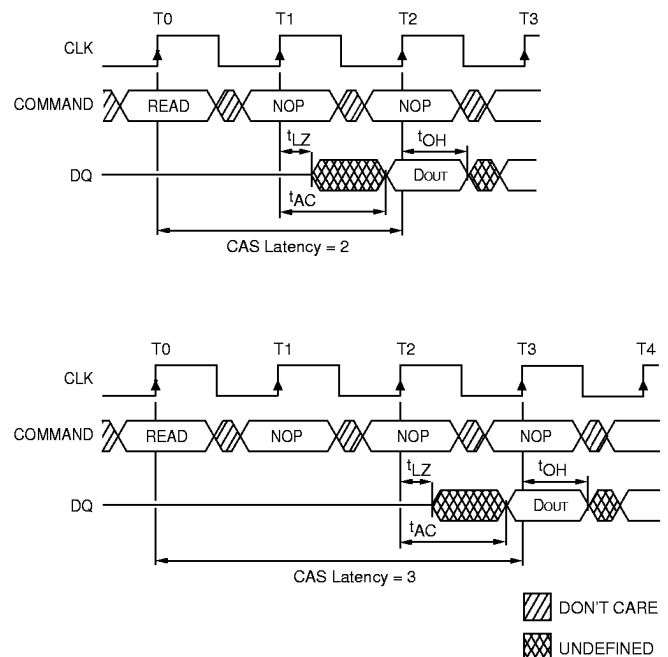
Figure 6 CAS LATENCY
