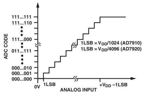
Figure 6. Transfer Characteristic
