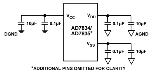
Figure 30. Power Supply Decoupling
