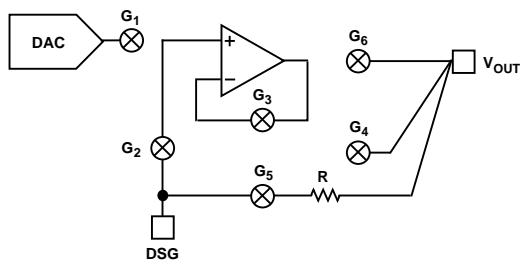
Figure 16. Output Stage with V_{DD} < 10 V
