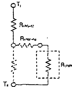
Fig. 6-1 Relationship of R_{th} , T_j and T_a
