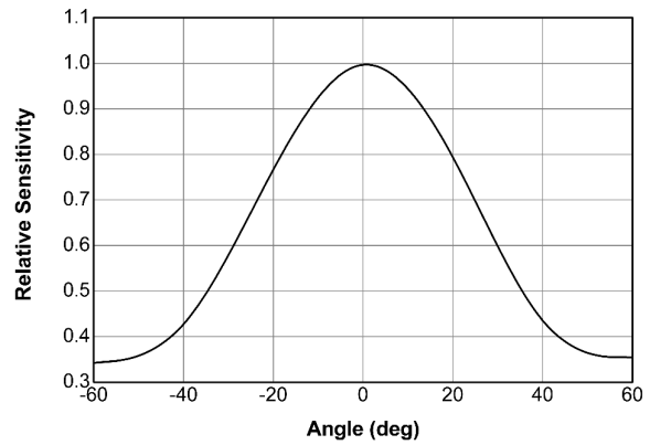
Fig.5 Relative Sensitivity vs. Angle
