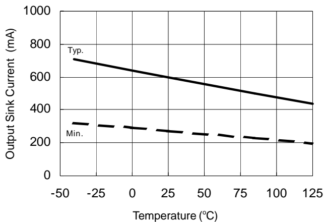
Figure 20A. Output Sink Current vs. Temperature
