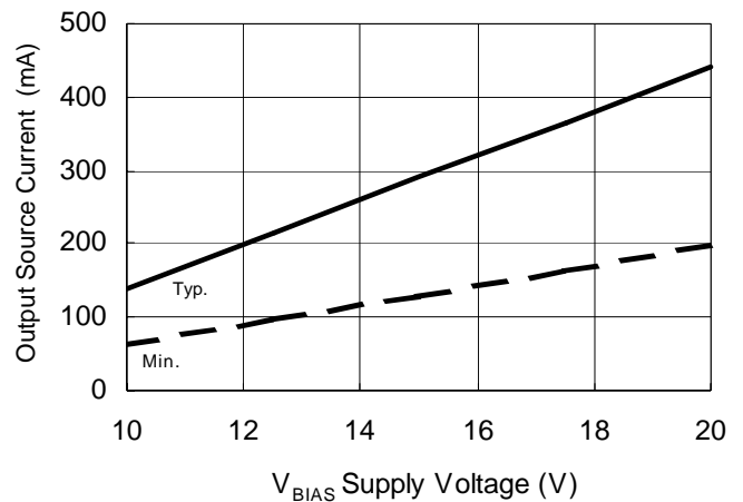
Figure 19B. Output Source Current vs. Supply Voltage
