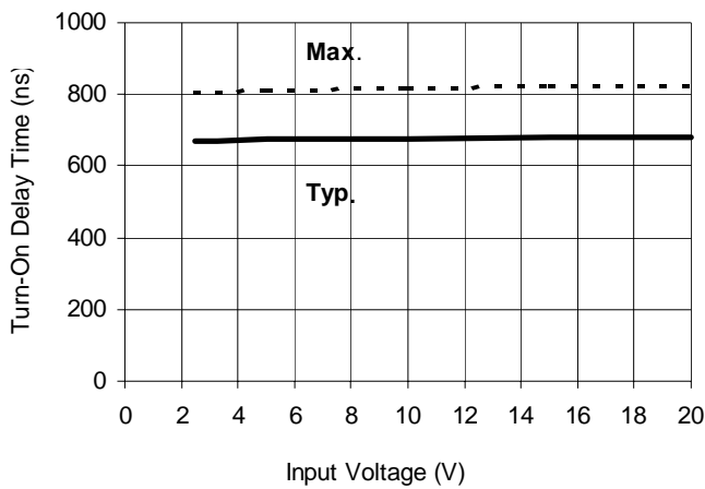
Figure 4C. Turn-On Time vs. Input Voltage
