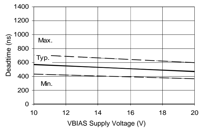
Figure 8B. Deadtime vs. Voltage
