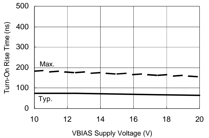
Figure 6B. Turn-On Rise Time vs. Voltage
