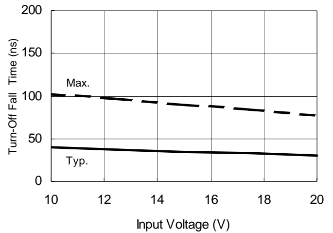
Figure 7B. Turn-Off Fall Time vs. Voltage
