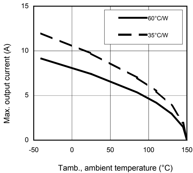
Figure 12 – Max. lout (A) Vs Tamb. (°C)
