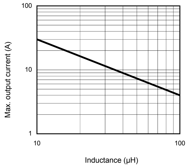
Figure 13 – Max. lout (A) Vs inductance (μH)
