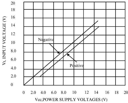
Figure 1. Input Voltage Range
