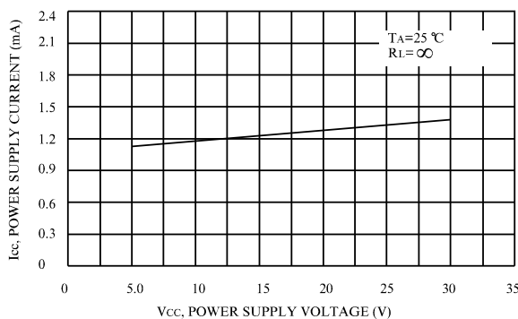
Figure 5. Power Supply Current versus Power Supply Voltage
