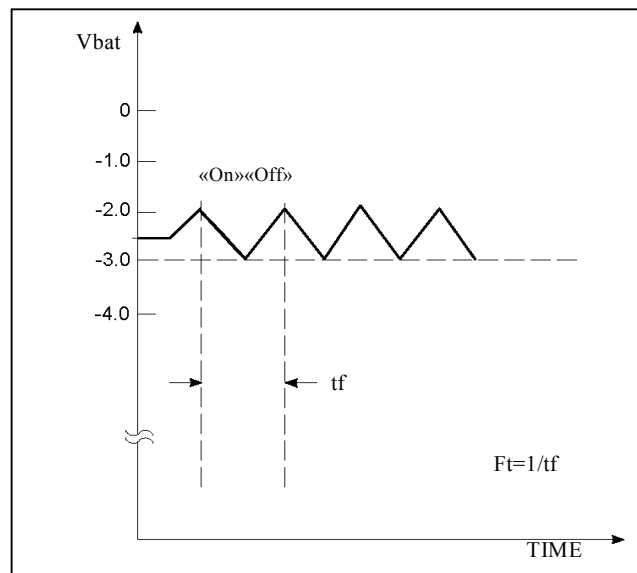
Figure 2 - One Defective Lamp Oscillator Timing Diagram
