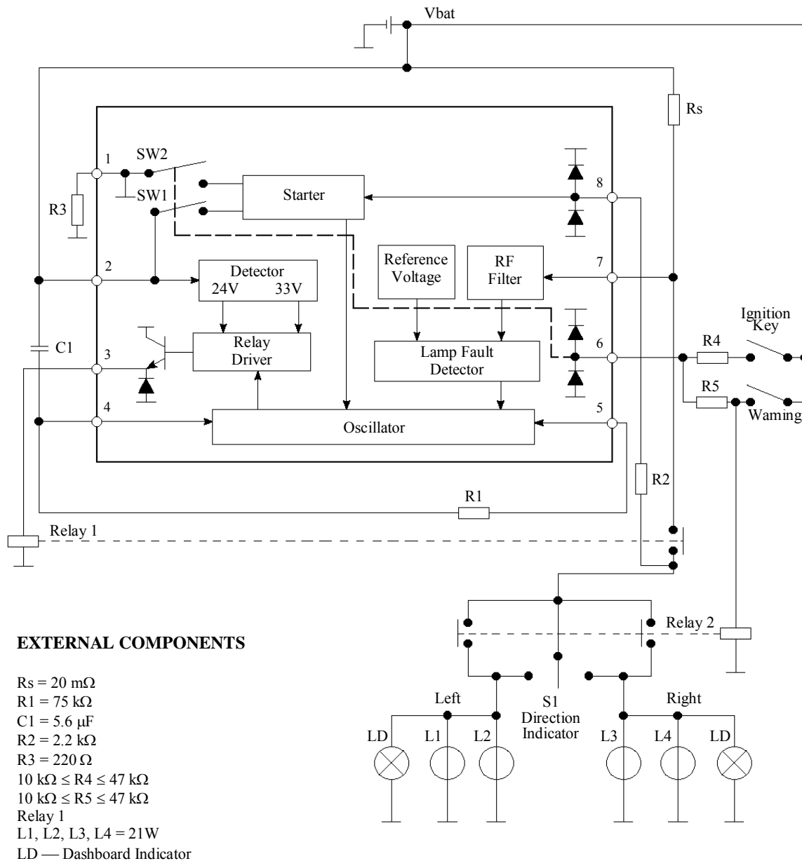
Figure 10. IL33193 Typical Application
