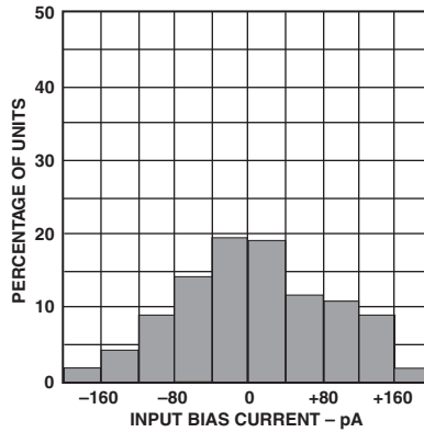
TPC 2. Typical Distribution of Input Bias Current
