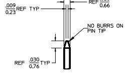
DETAIL X SCALE 5:1 SEE NOTE 10
