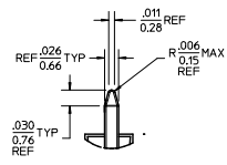
DETAIL Y SCALE 5:1 SEE NOTE 10
