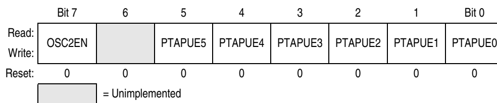
Figure 11-4. Port A Input Pullup Enable Register (PTAPUE)
