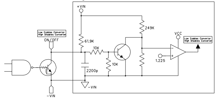
Figure 3: Active Low
