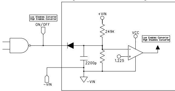
Figure 2: Active High
