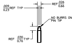
DETAIL X SCALE 5:1 SEE NOTE 10
