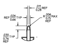
DETAIL Y SCALE 5:1 SEE NOTE 10
