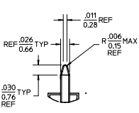
DETAIL Y SCALE 5:1 SEE NOTE 10
