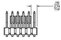
REMOVED POLARIZING WALL OPTION
