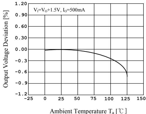
Fig.4 V_O vs T_a
