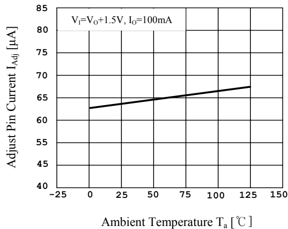
Fig.6 I_{Adj} vs T_a
