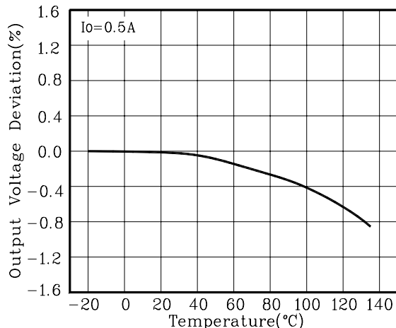
Fig. 6 Temperature Stability
