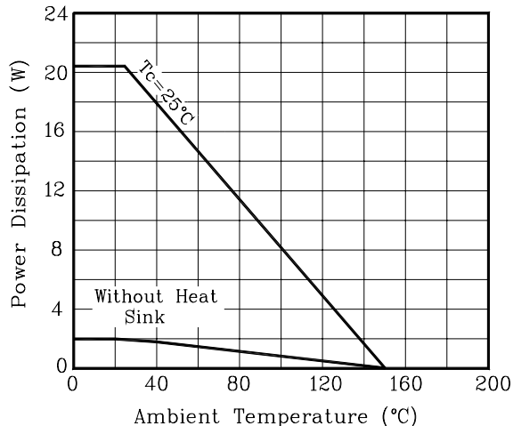
Fig. 8 P_D vs. T_a
