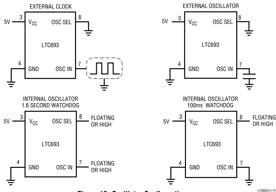
Figure 12. Oscillator Configurations
