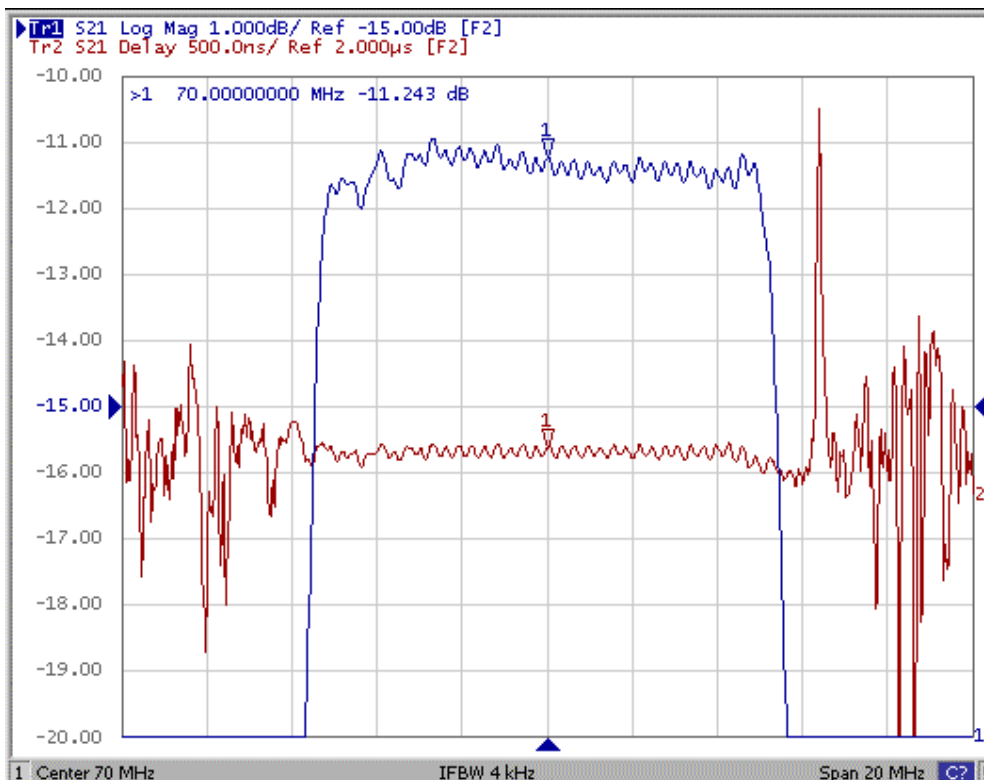
Fig2. Horizontal: 2MHz/Div Vertical: 500nec/Div
