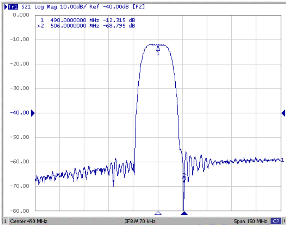
(1) S21 Response:(span 100MHz)
