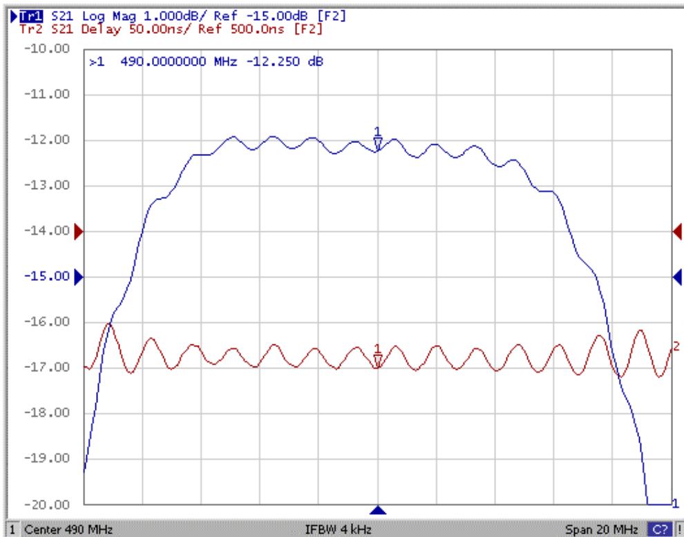
(2) Passband of Response: (span: 20MHz)
