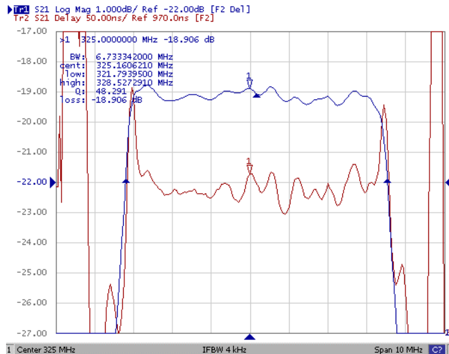
Fig2. Horizontal: 1MHz/Div Vertical: 1dB/Div 1MHz/Div Vertical: 50nS/Div
