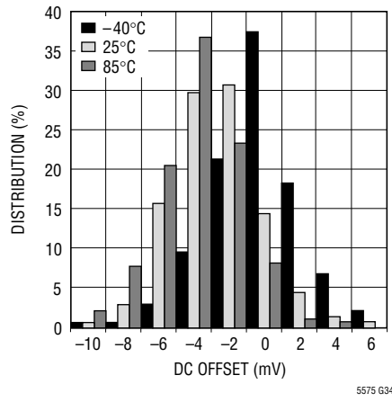
Q-Output DC Offset Voltage Distribution vs Temperature
