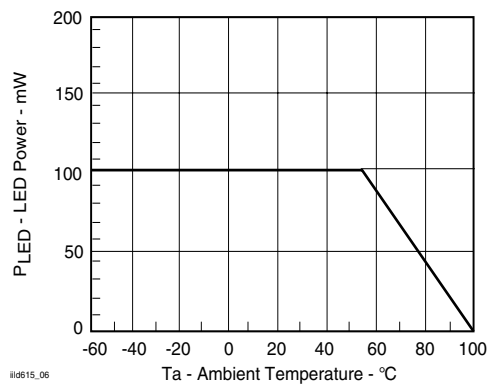
Figure 6. Maximum LED Power Dissipation
