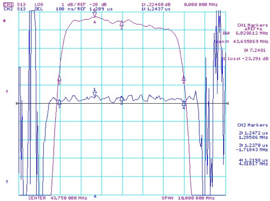
Figure-2 S21 Response(Pass Band/SPAN=10MHz)
