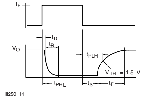
Fig. 14 - Switching Timing
