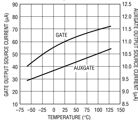
GATE, AUXGATE Output Source Current vs Temperature
