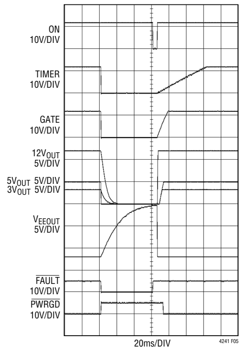
Figure 5. Short-Circuit on 5V Followed by Circuit Breaker Reset
