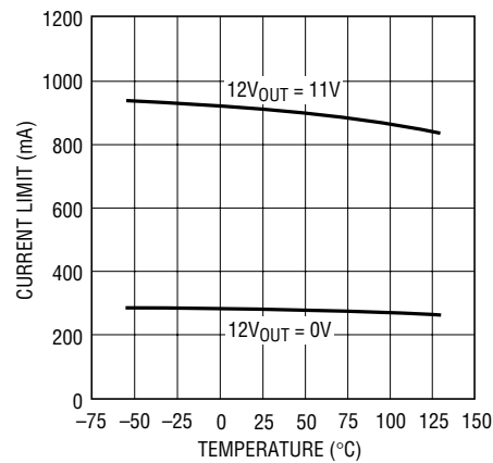
12V IN Current Limit vs Temperature
