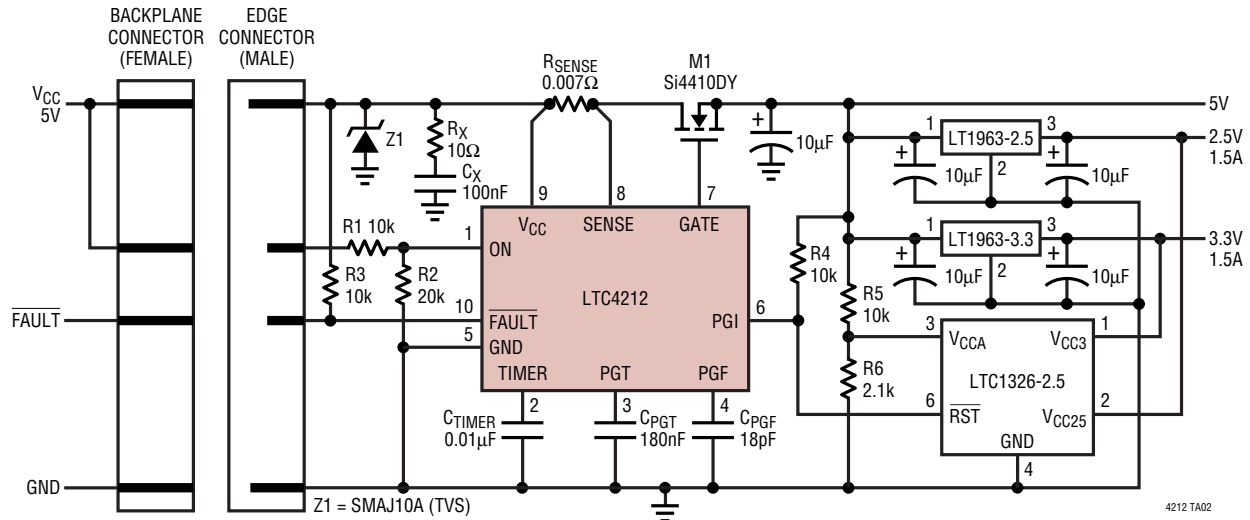
Monitoring DC/DC Converters with the LTC1326-2.5 Supply Monitor
