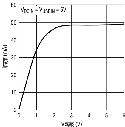
PWR Pin I-V Curve
