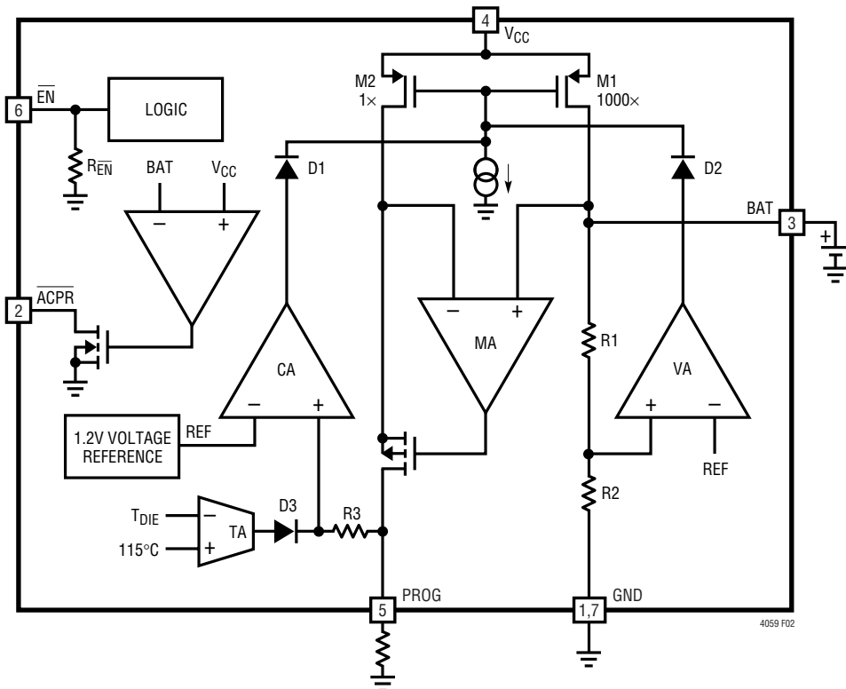
Figure 2 (LTC4059A)
