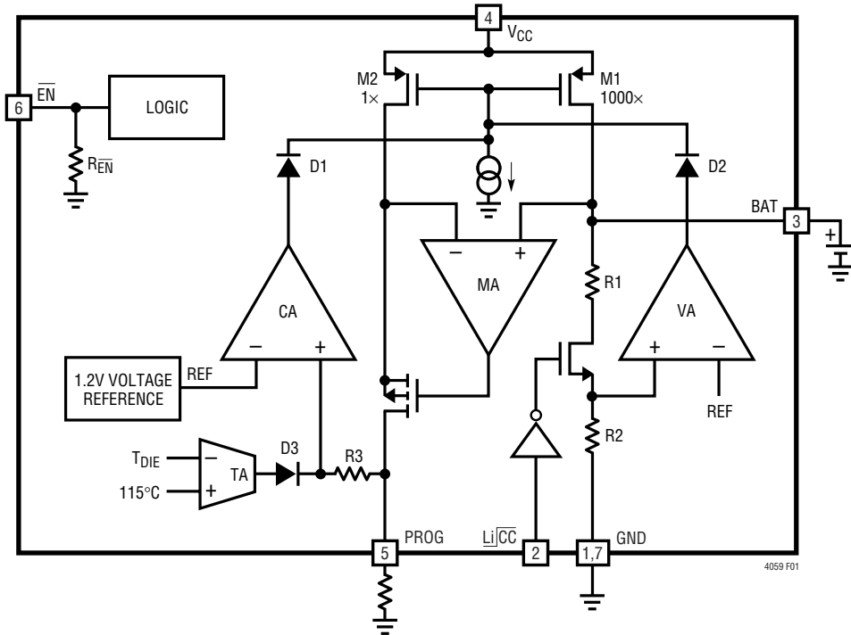
Figure 1 (LTC4059)
