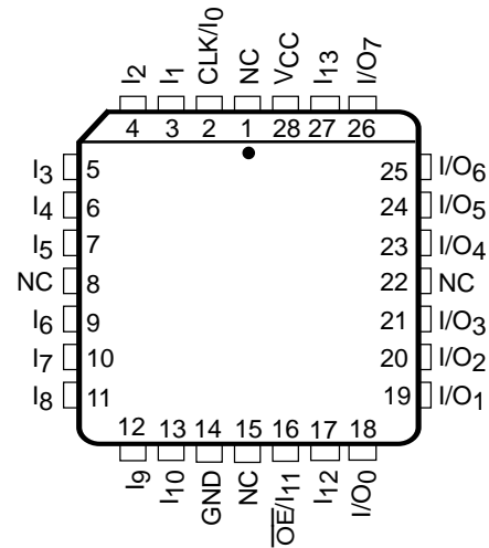
PLCC/LCC
