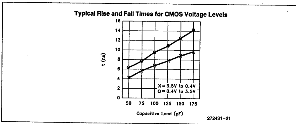
Figure 19. CMOS Level Rise and Fall Times for Output Buffers
