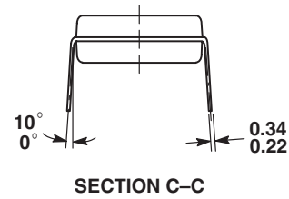
Figure 20-5. 32-Pin SDIP (Case #1376)
