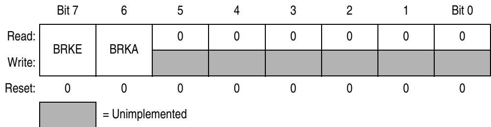
Figure 18-3. Break Status and Control Register (BRKSCR)
