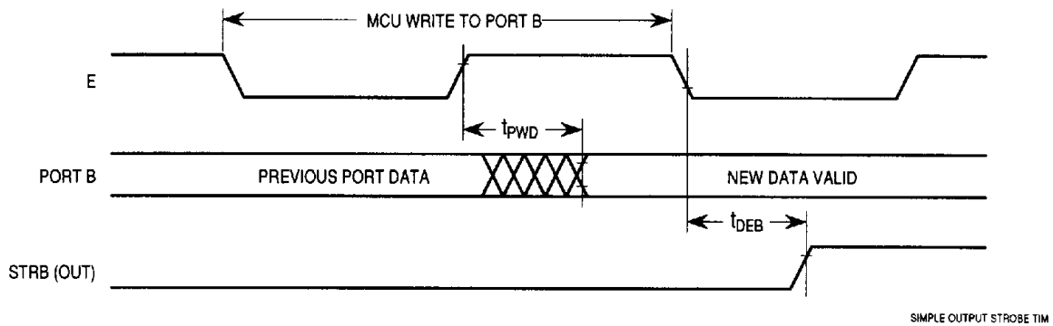
Figure A-10. Simple Output Strobe Timing Diagram
