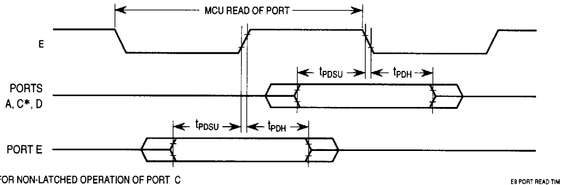
Figure A-7. Port Read Timing Diagram
