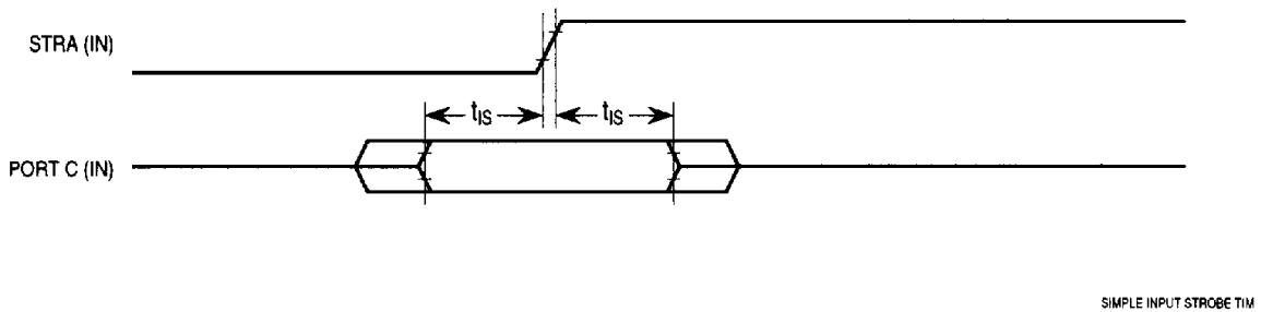
Figure A-9. Simple Input Strobe Timing Diagram
