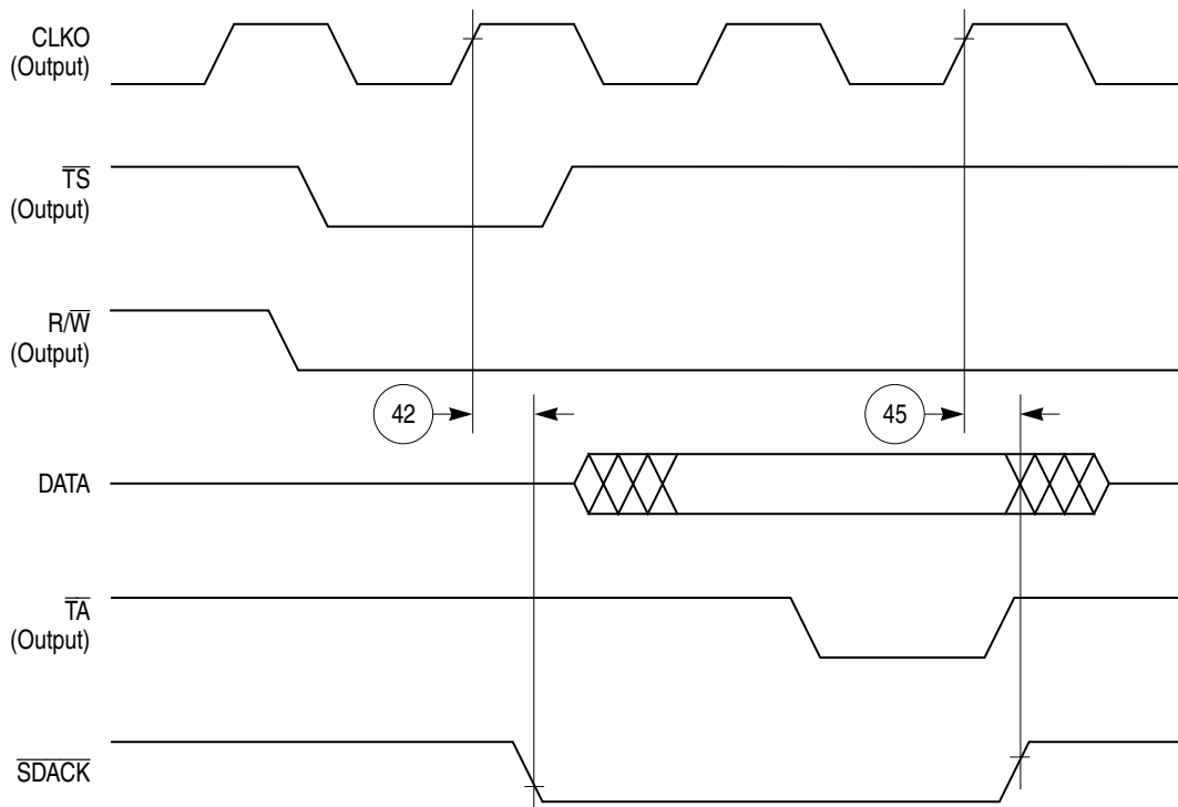
Figure 49. SDACK Timing Diagram—Peripheral Read, Internally-Generated TA
