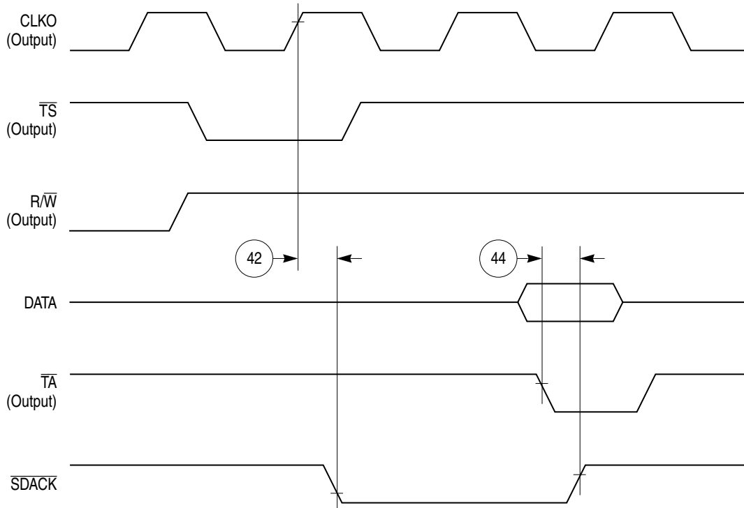
Figure 48. SDACK Timing Diagram—Peripheral Write, Internally-Generated TA
