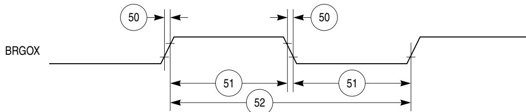
Figure 50. Baud Rate Generator Timing Diagram
