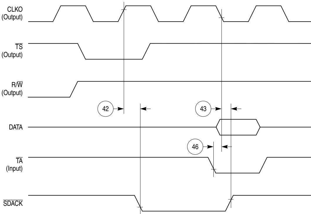
Figure 47. SDACK Timing Diagram—Peripheral Write, Externally-Generated \overline{\text{TA}}
