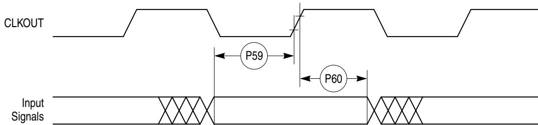
Figure 30. PCMCIA Input Port Timing
