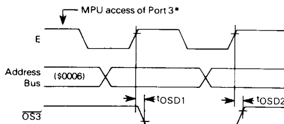
FIGURE 4 — PORT 3 OUTPUT STROBE TIMING (MC6801 SINGLE-CHIP MODE)
