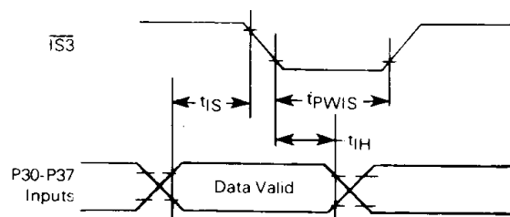
FIGURE 5 — PORT 3 LATCH TIMING (MC6801 SINGLE-CHIP MODE)
