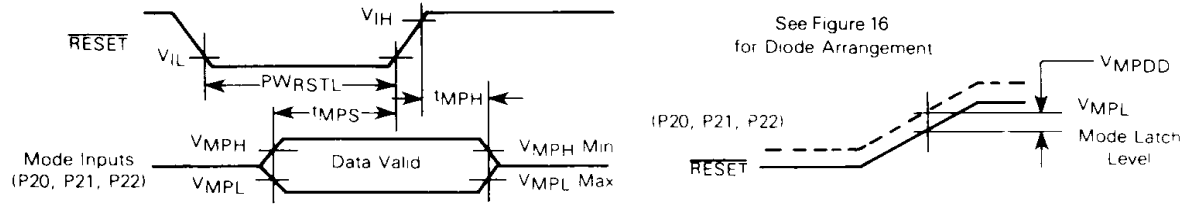
FIGURE 15 — MODE PROGRAMMING TIMING
