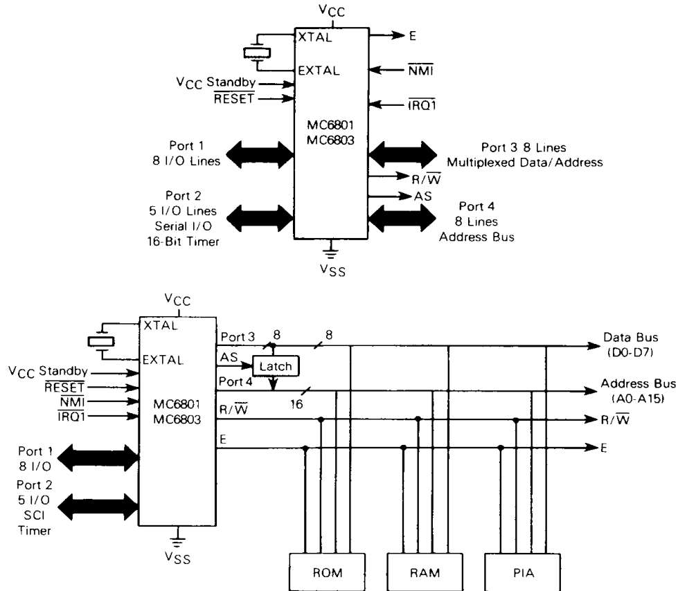
FIGURE 13 — EXPANDED MULTIPLEXED CONFIGURATION
