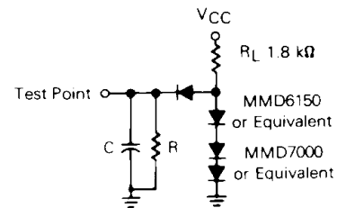
FIGURE 8 — TIMING TEST LOAD PORTS 1, 2, 3, 4
