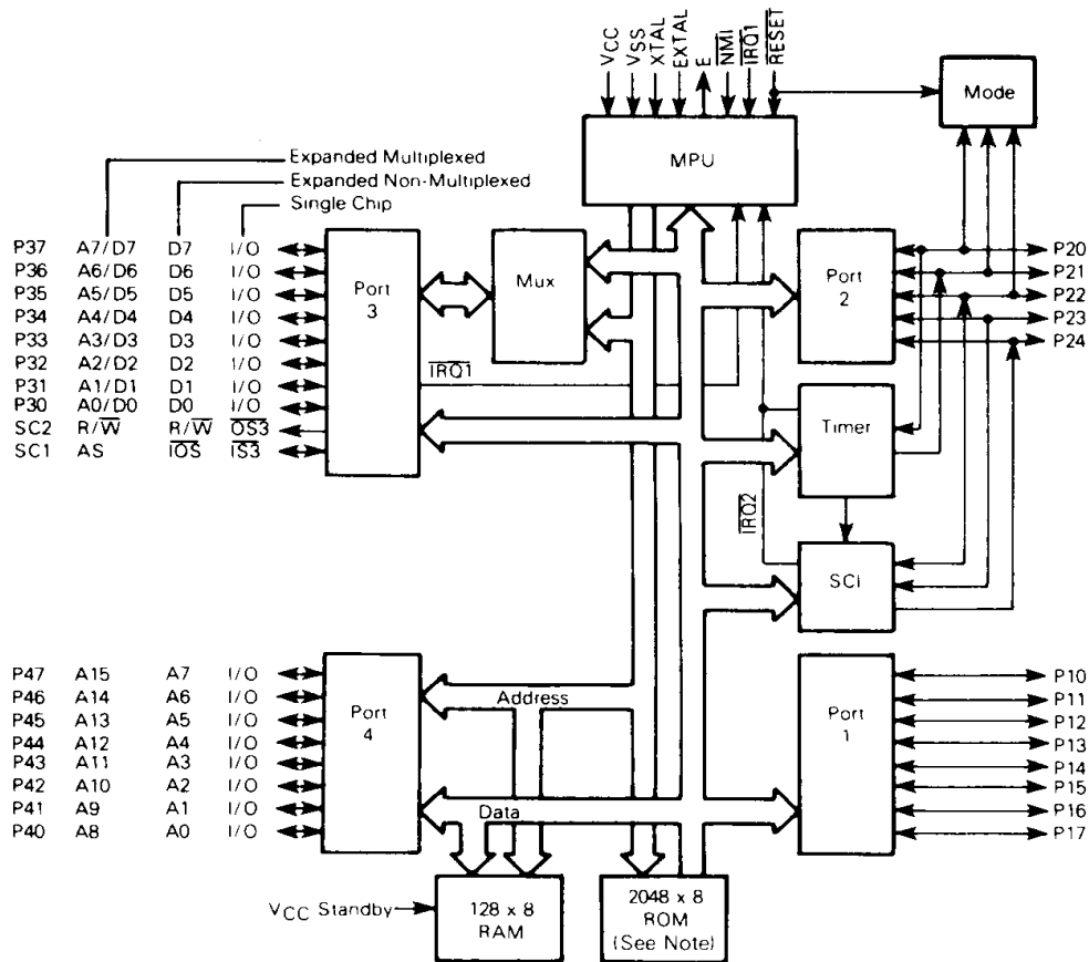
FIGURE 1 — M6801 MICROCOMPUTER FAMILY BLOCK DIAGRAM
