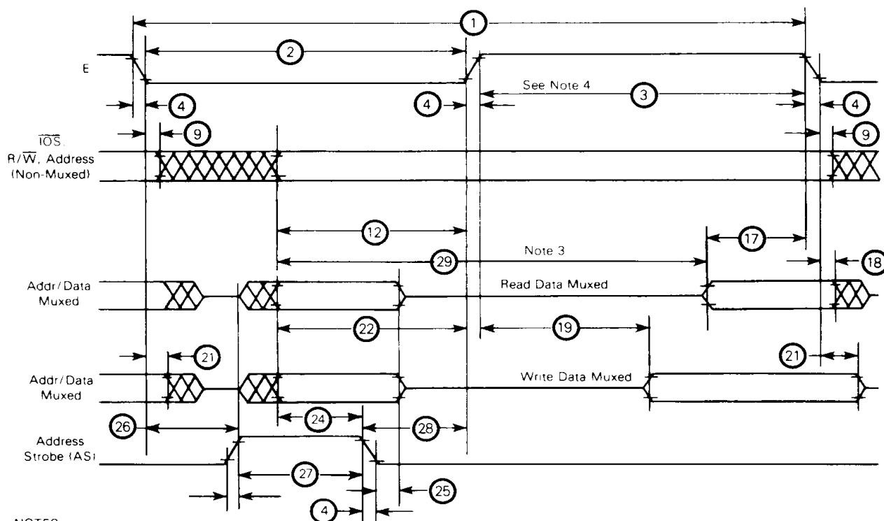
FIGURE 6 — BUS TIMING
