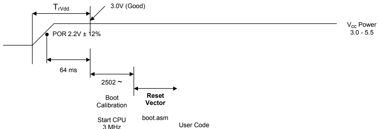
Figure 30: Execution Reset
