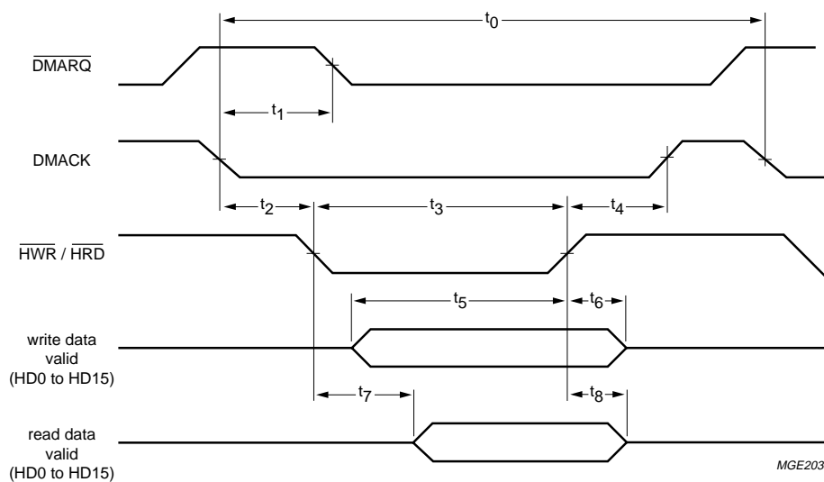
Fig.15 Single-word DMA transfer.
