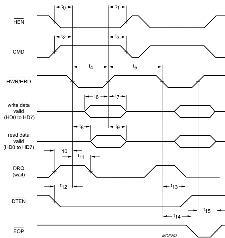
Fig.19 DRQ control data transfer.
