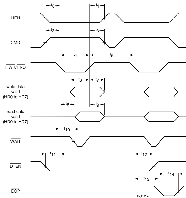
Fig.18 \overline{\text{WAIT}} control and data transfer.
