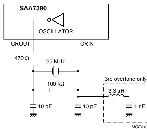
Fig.25 Crystal oscillator circuit.
