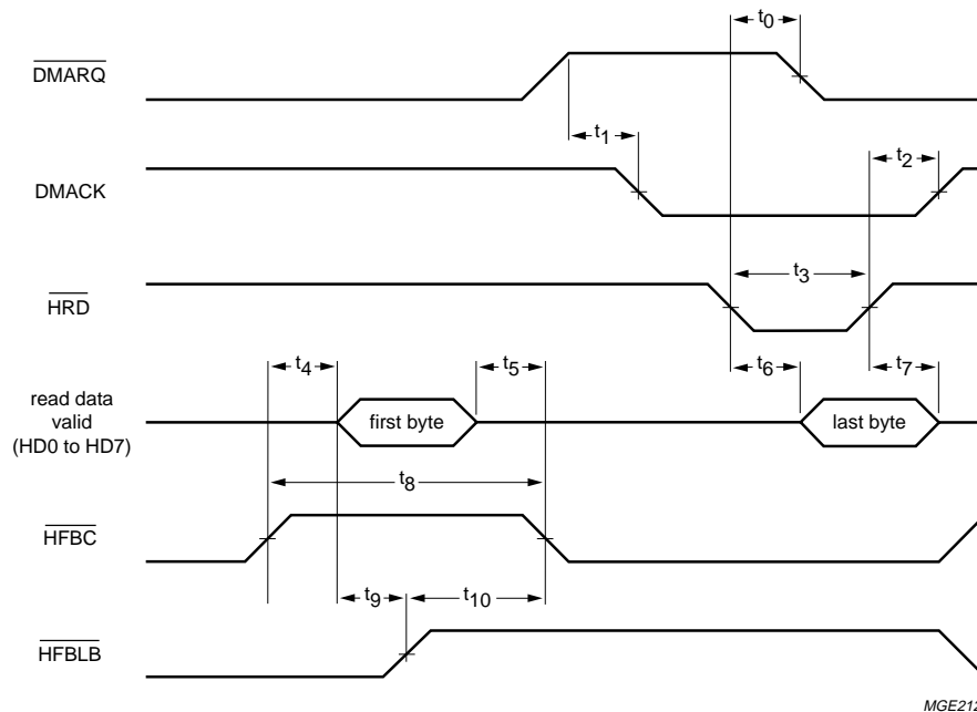
Fig.24 Pseudo 16-bit DMA read transfer.
