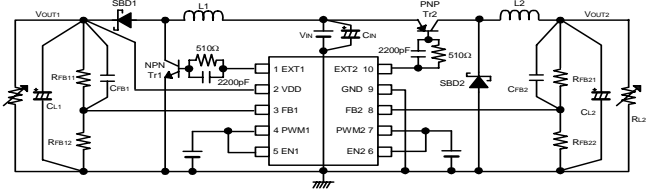
Circuit 2
