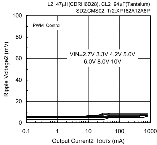
FOSC=180kHz, VOUT2=3.3V
