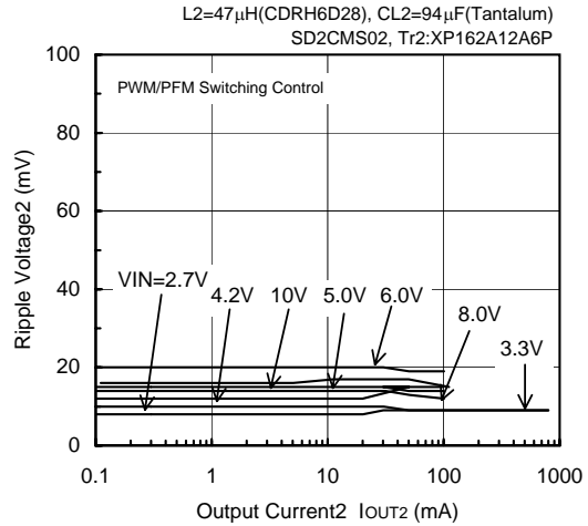
FOSC=180kHz, VOUT2=1.0V
