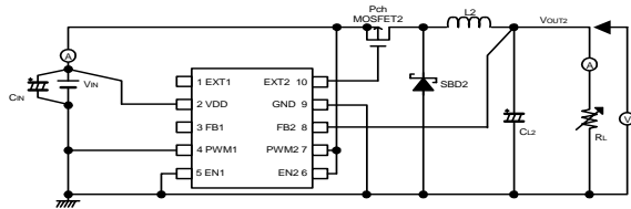
Circuit 7
