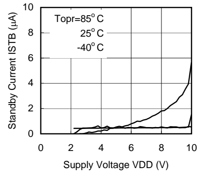
XC9502B092 (180kHz)
