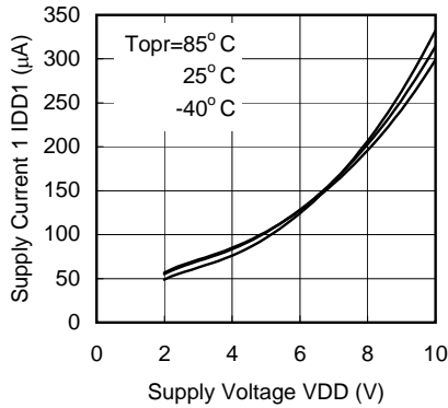
(9) Supply Current 1-2 vs. Supply Voltage
