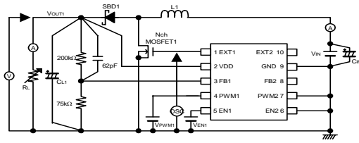
Circuit 6
