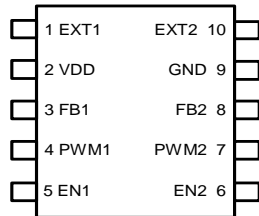
MSOP-10 (TOP VIEW)
