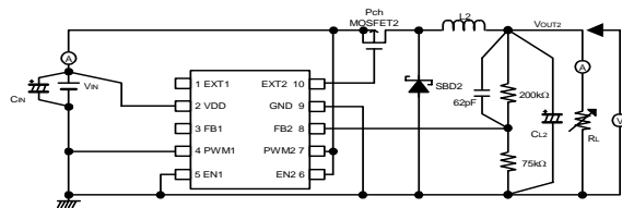
Circuit 8
