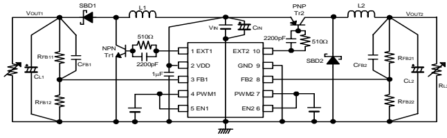
Circuit 1
