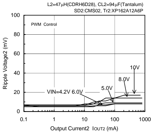
FOSC=180kHz, VOUT2=3.3V
