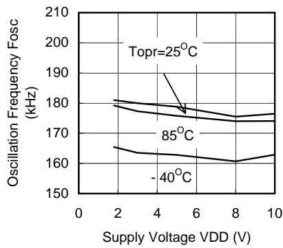
XC9502B092 (180kHz)
