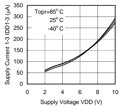
(12) Supply Current 2 vs. Supply Voltage
