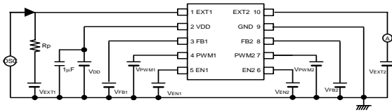
Circuit 7
