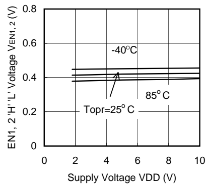
XC9502B092 (180kHz)
