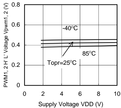
XC9502B092 (180kHz)
