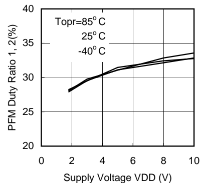
XC9502B092(180kHz)
