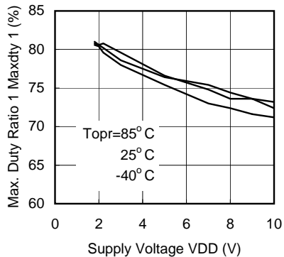
XC9502B092 (180kHz)
