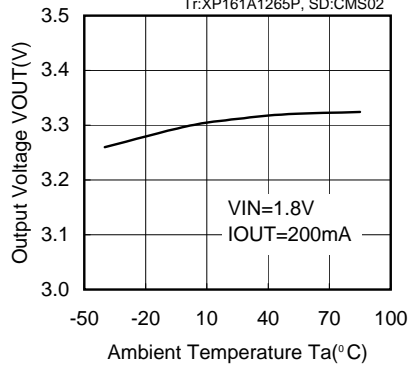
XC9502B093(300kHz)
