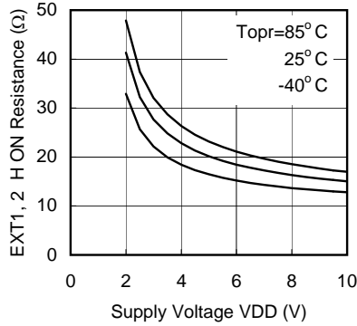
XC9502B092 (180kHz)
