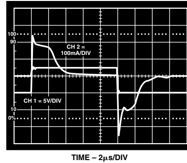
Figure 6. Scope Photo of the V_{\text{COM}} Instantaneous Peak Current
